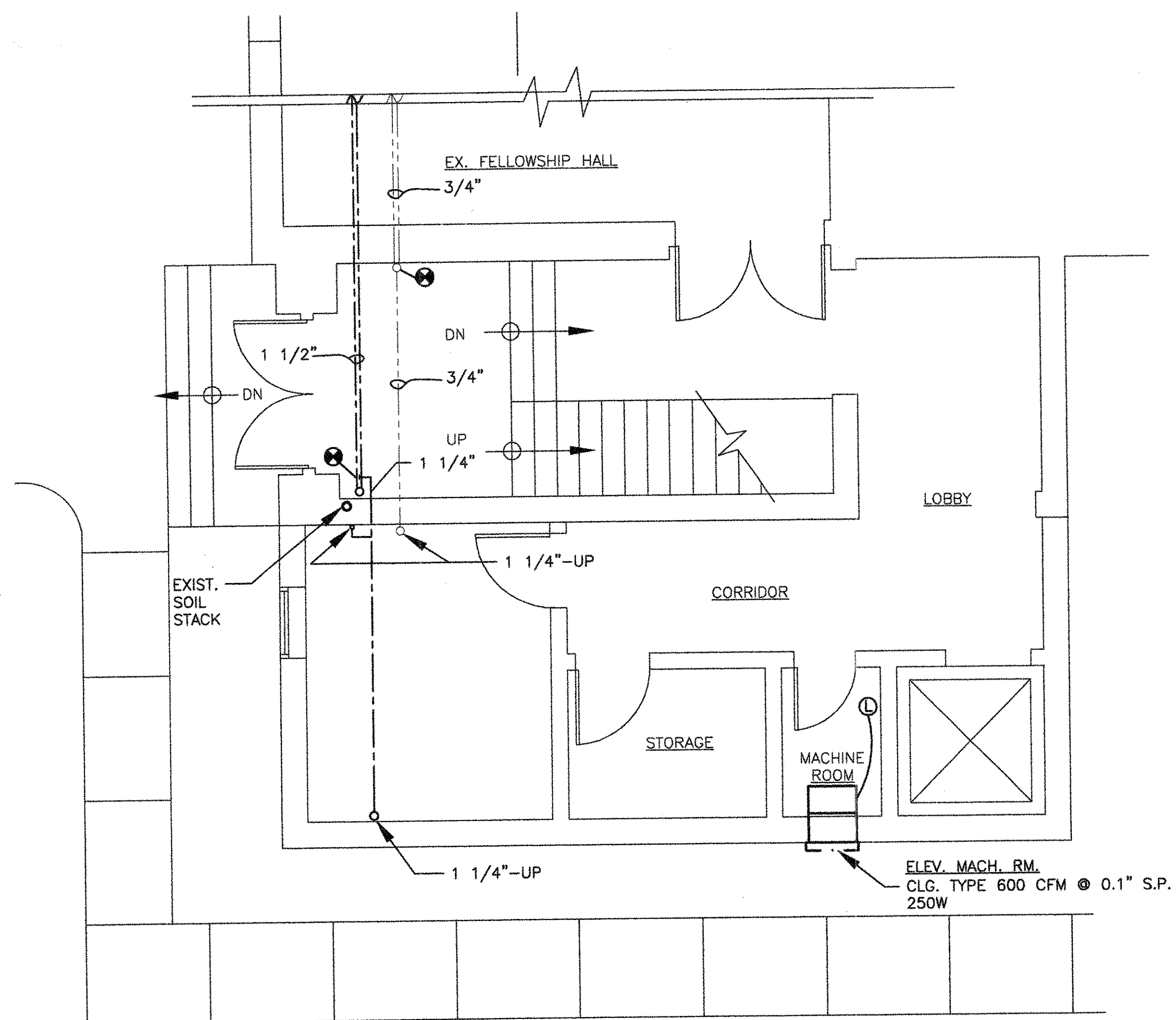
1 LOWER LEVEL PLAN MP.1 SCALE: 1/4" = 1'-0"
