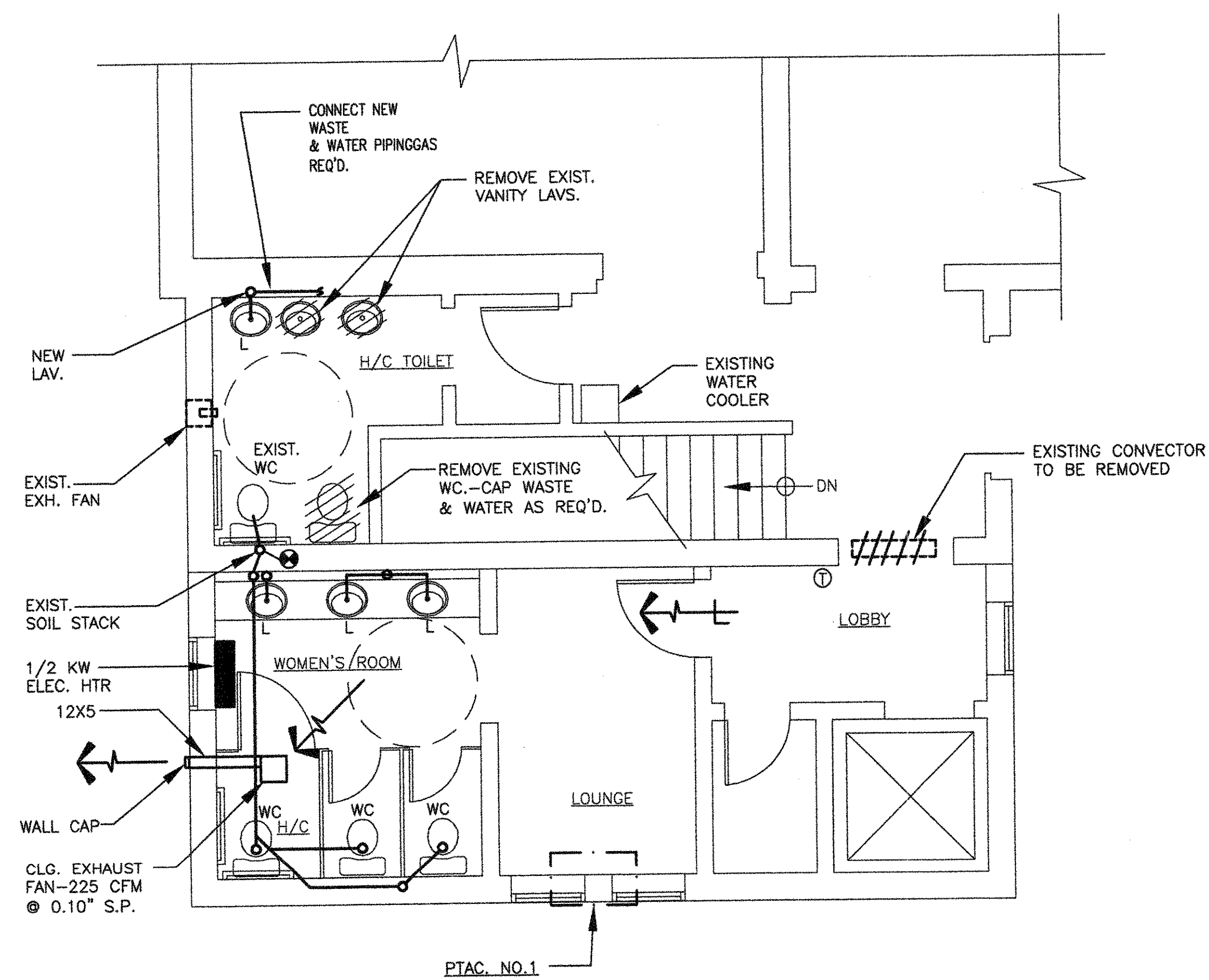
2 UPPER LEVEL PLAN MP.1 SCALE: 1/4" = 1'-0"
