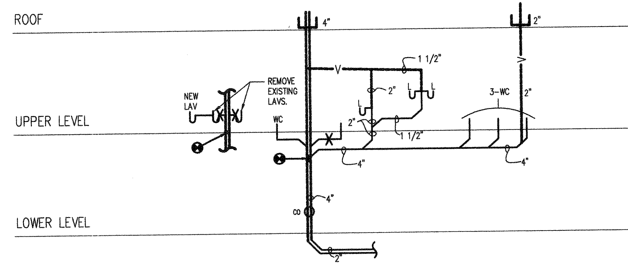
WATER RISER DIAGRAM NOT TO SCALE
