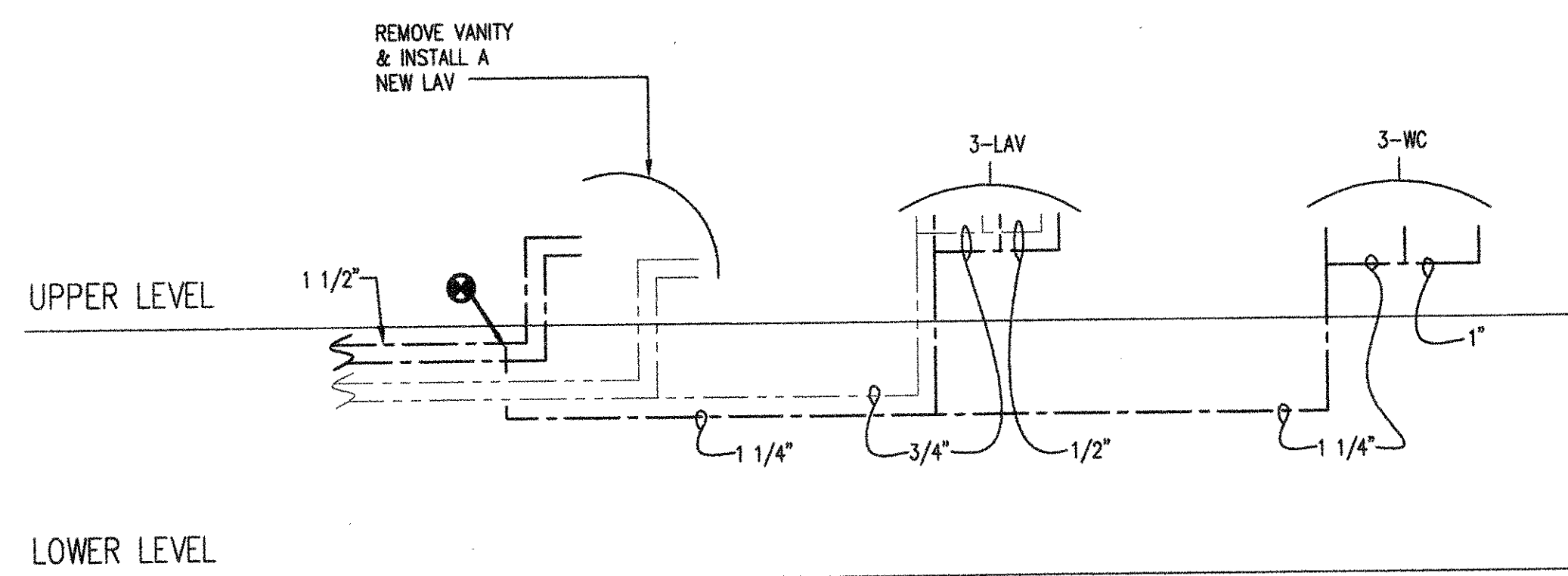
DRAINAGE DIAGRAM NOT TO SCALE
